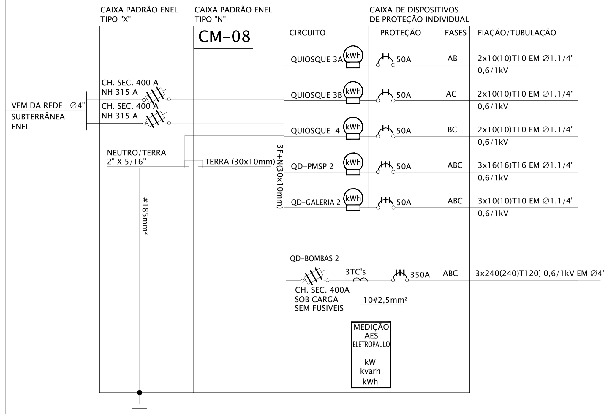
DIAGRAMA UNIFILAR DO CM-08
